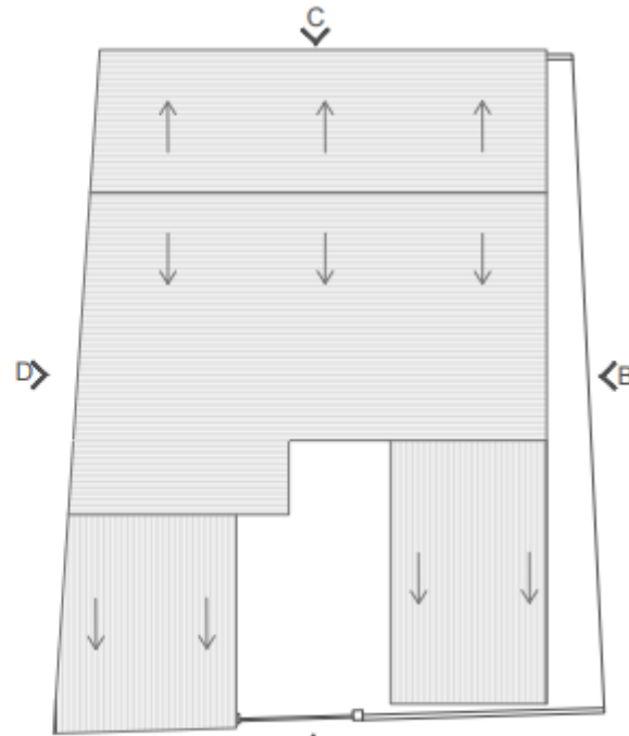
ROOF PLAN
